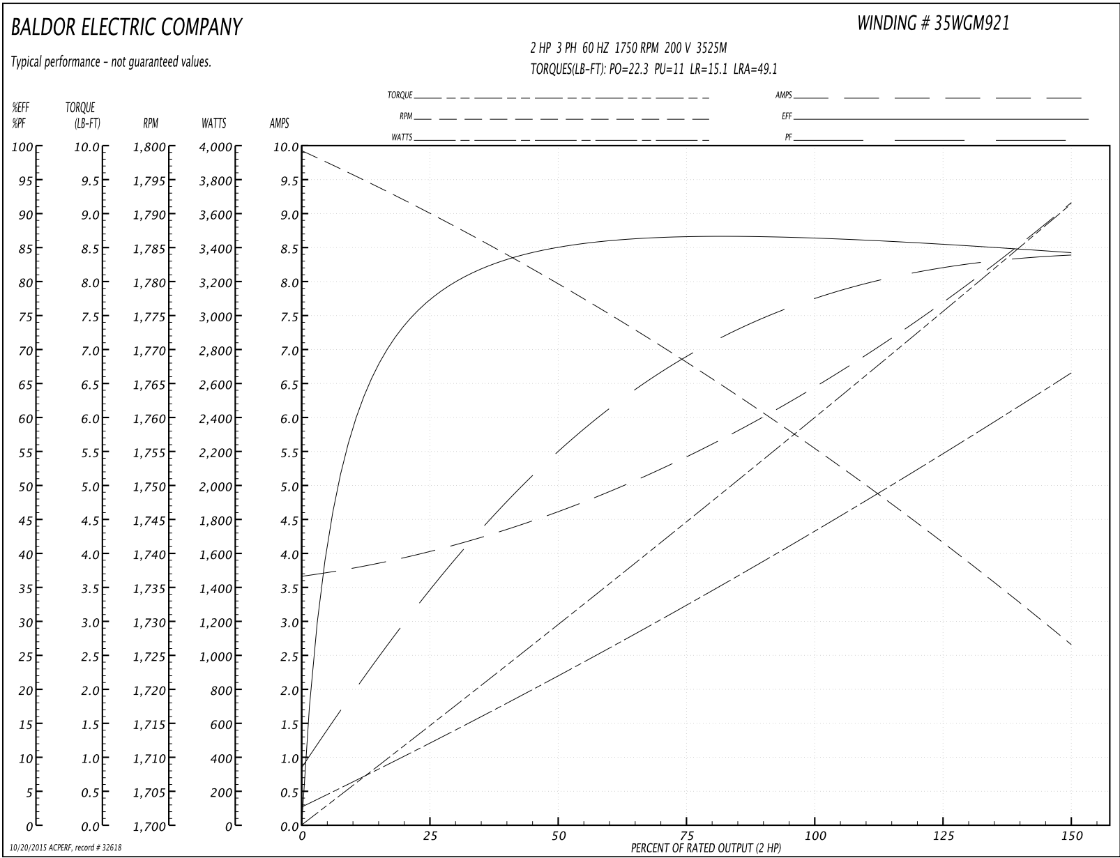
Performance Graph at 200V, 60Hz, 2.0HP Typical performance - Not guaranteed values
