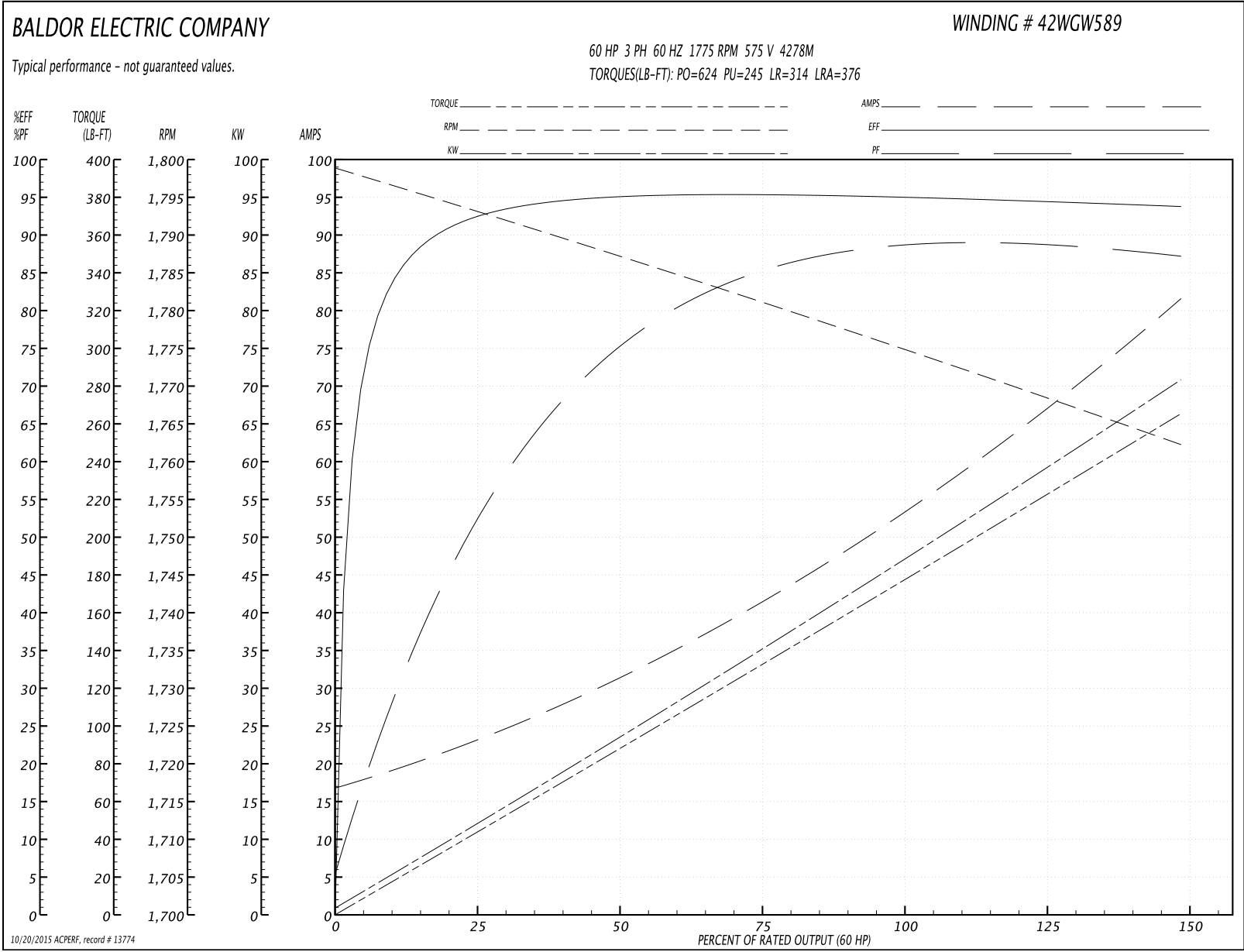
Performance Graph at 575V, 60Hz, 60.0HP Typical performance - Not guaranteed values
